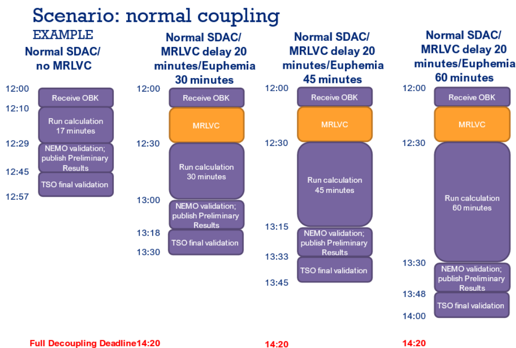
Figure 9: 15-minute MTU timings impact on partial coupling
